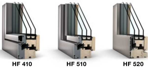
Holz-Aluminium-Fenster
